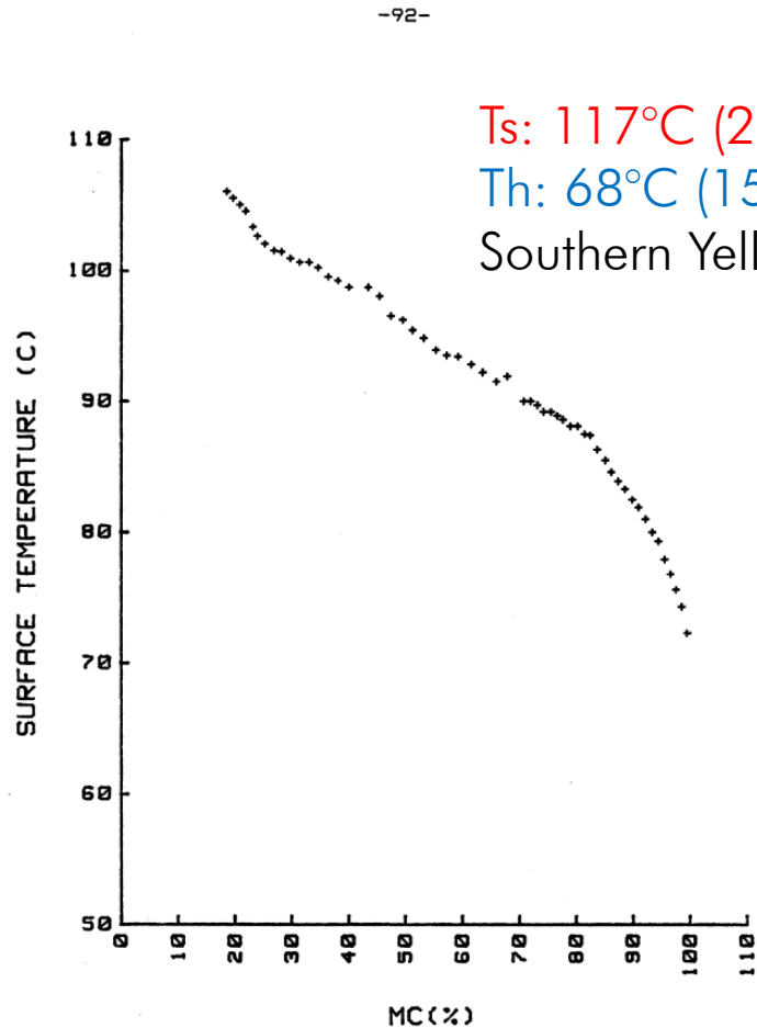
Fig.12 Temperature near the surface of the wood versus moisture content, Experiment 1.
